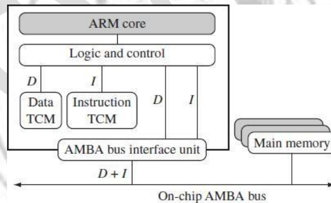
Figure: Harvard Architecture with TCMs
