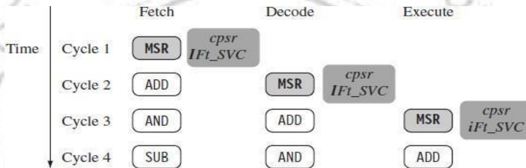
Figure: ARM Instruction Sequence
