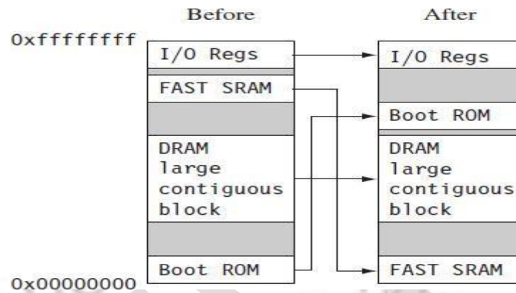
Figure: Memory Remapping
