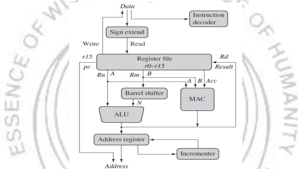
Figure: ARM Core dataflow Model
