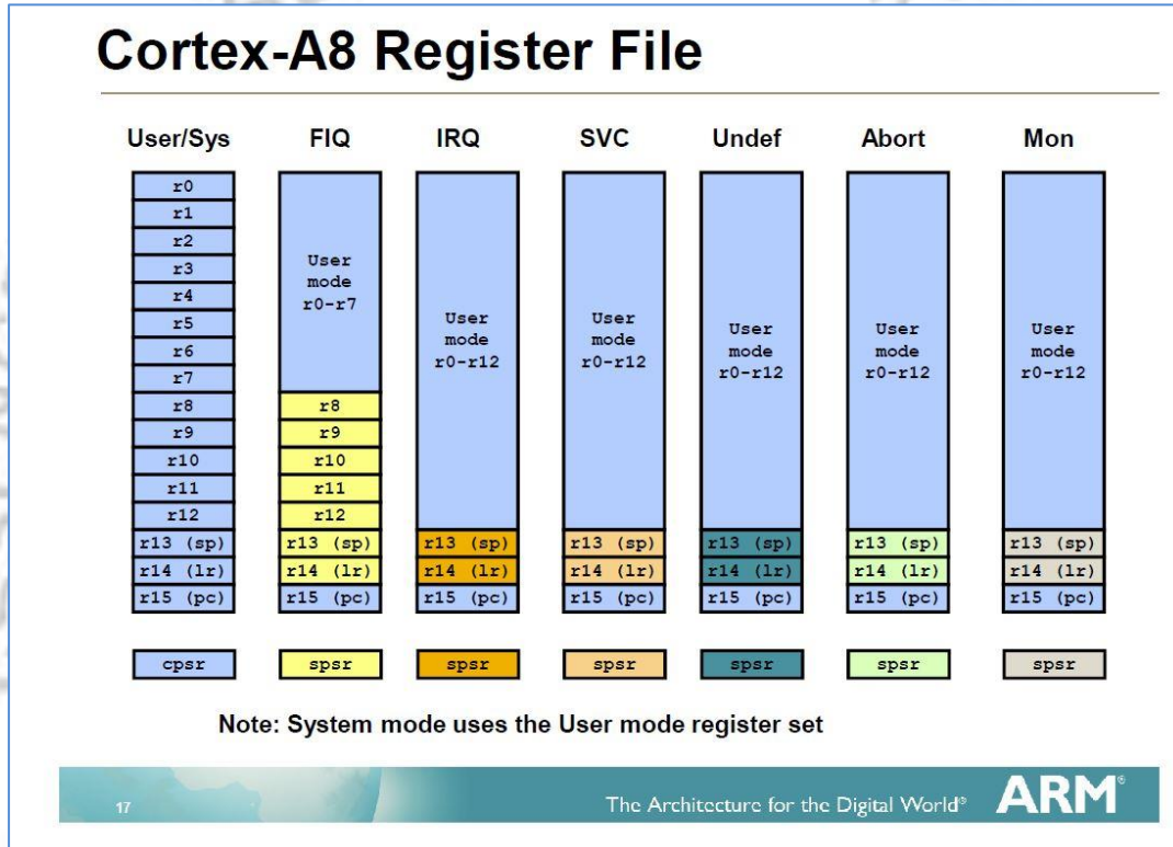
Figure: Complete ARM Register Set
